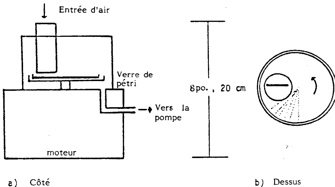
FIGURE 9 ET FIGURE 10: SLIT SAMPLER
